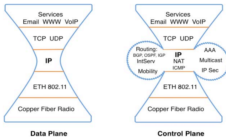
Figure 1 – Current Internet Architecture
