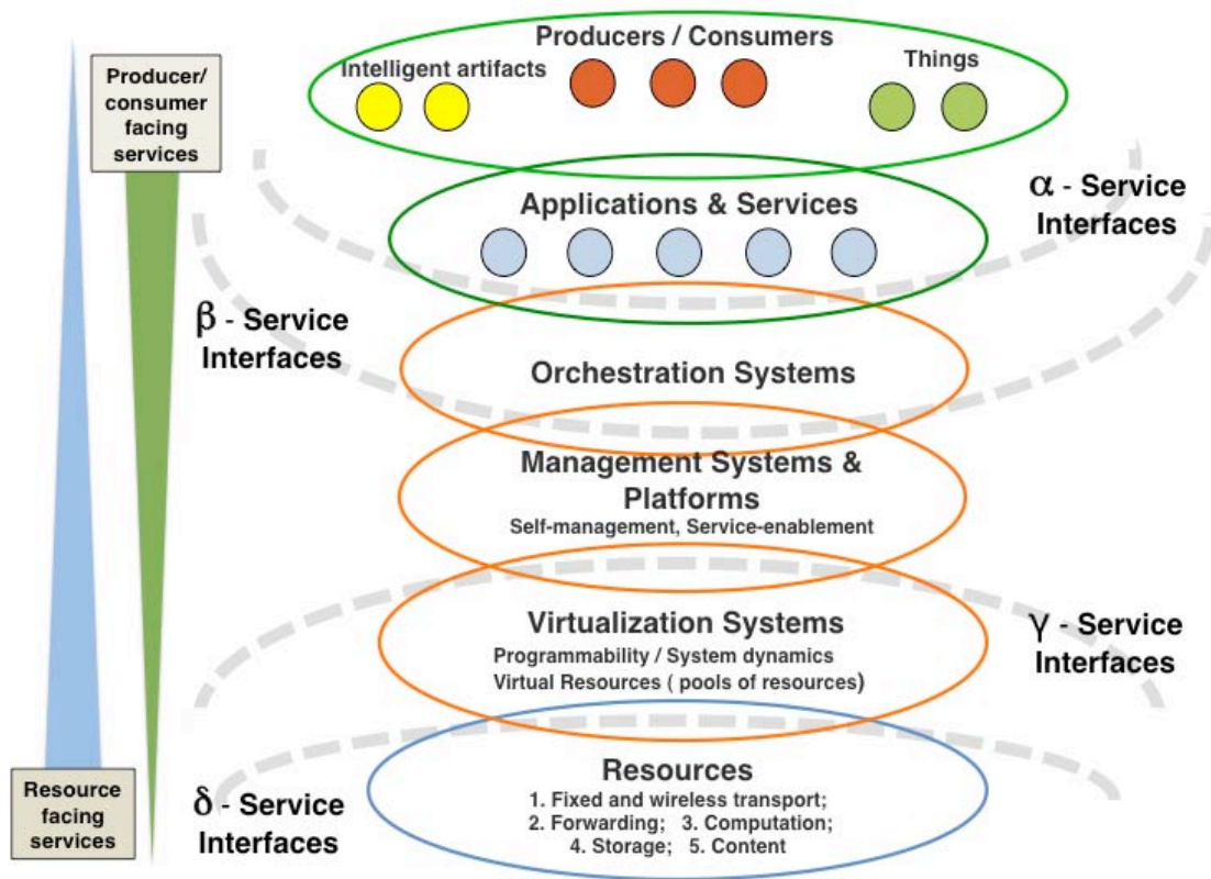
Figure 2 – MANA architectural model
